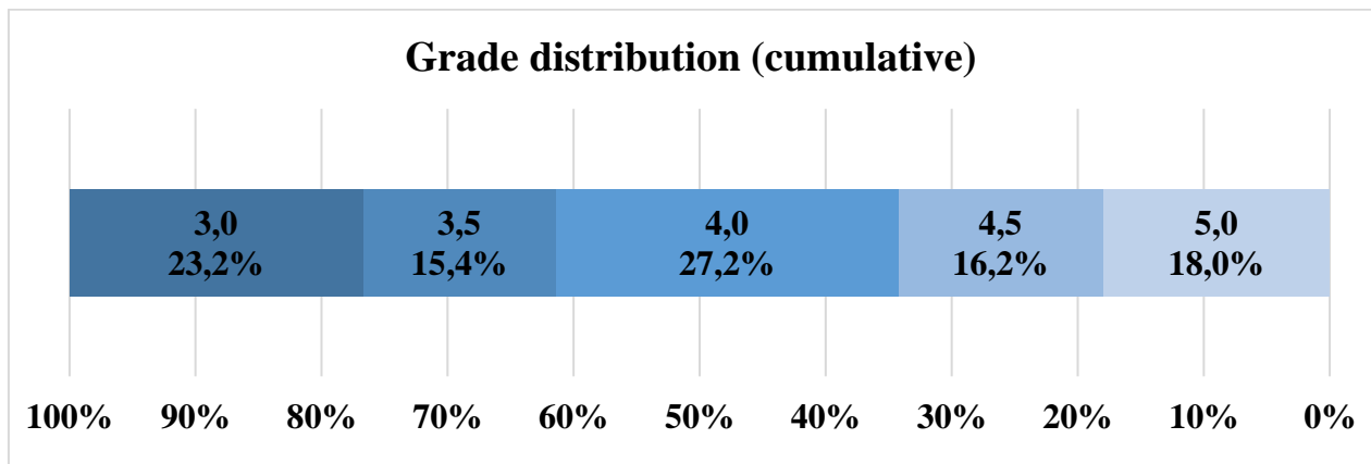
Fig. 1. Grade distribution (cumulative)
